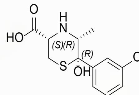
Bupropion SRR-Isomer [Bupropion Thio morpholine SRR Isomer, S,R,R-Thiomorpholine derivative] DCTI-C-1259
