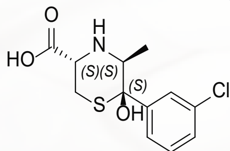
Bupropion SSS-Isomer [Bupropion Thio morpholine SSS isomer, S,S,S- Thiomorpholine derivative] DCTI-C-1225
